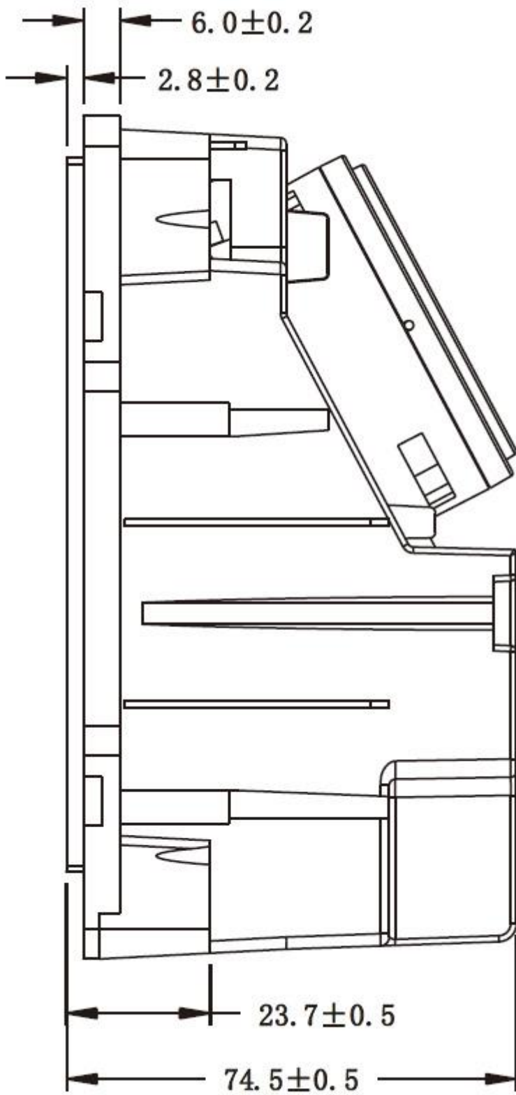
Figure 2-3 Dimensions (with stand)
